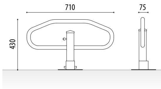
Open-close detail of the manual barrier for vehicle passage.
